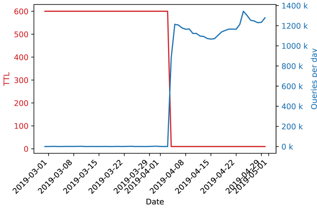
Figure 7: TTL decrease from 600 to 10 seconds on xmsecu.com leading to a massive increase in queries.
